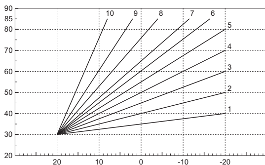
fig. 14- Compensation curves
