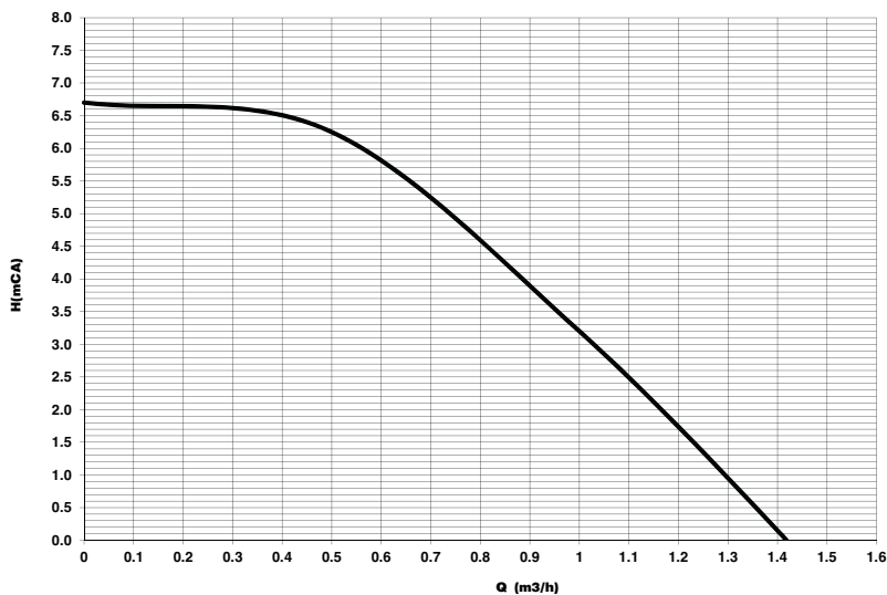
fig. 44- Residual head available for system
