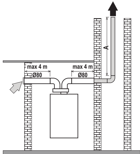
fig. 25- Layout for ducting only with flexible pipe
