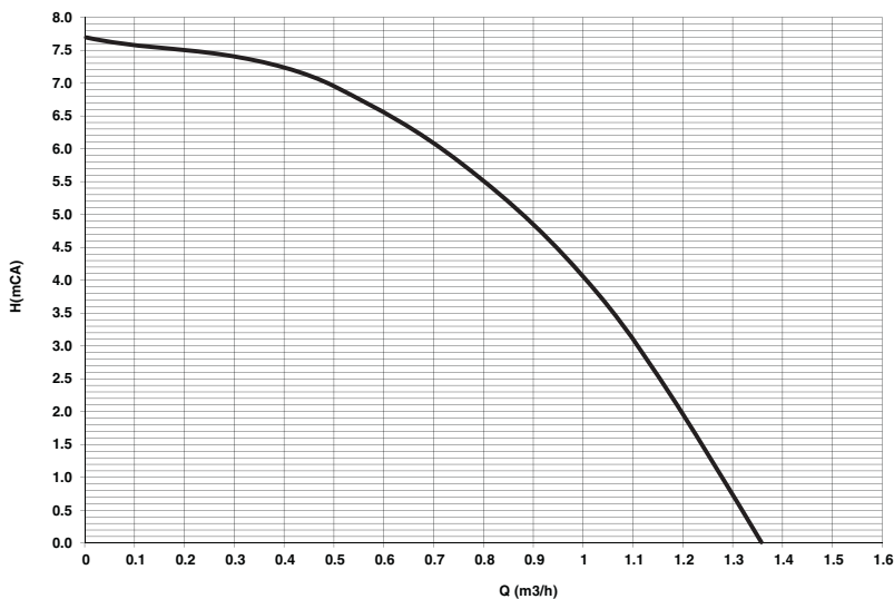
fig. 45- Residual head available for system
